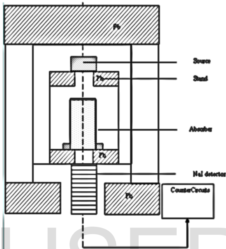
Fig. 1 - Experimental Arrangement
